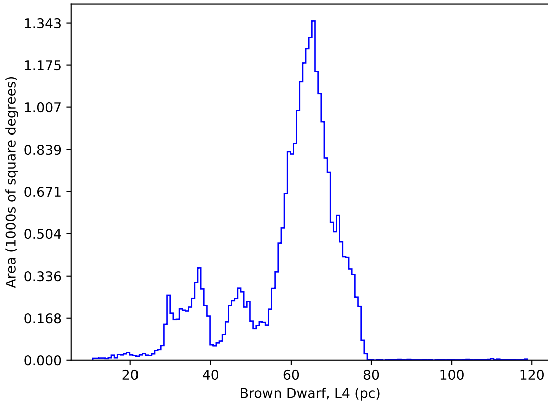
ddf_loaded_half_fl1_v3.4_10yrs : Brown Dwarf, L4
