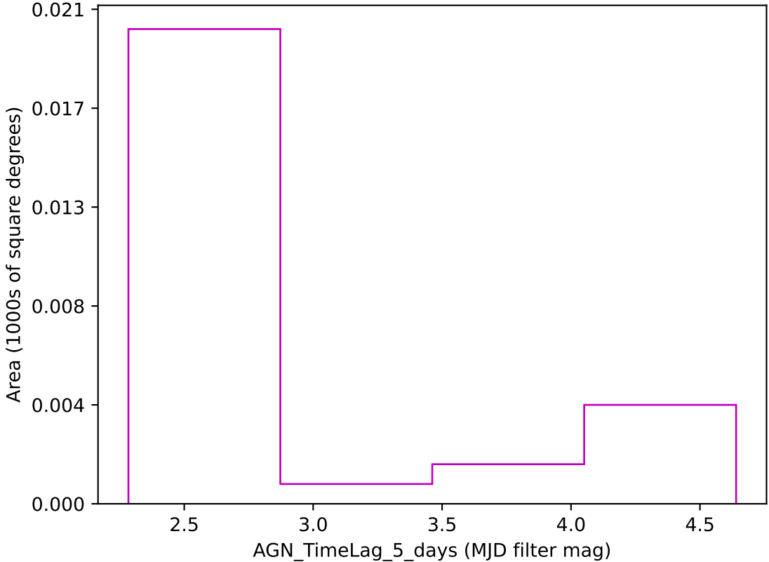
ddf_loaded_half_fl1_v3.4_10yrs z band: AGN_TimeLag_5_days
