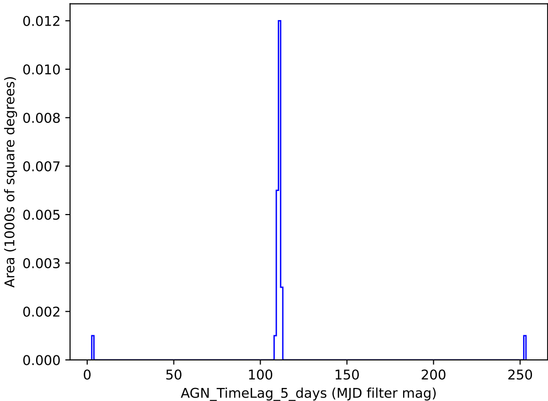
ddf_loaded_half_fl1_v3.4_10yrs y band: AGN_TimeLag_5_days
