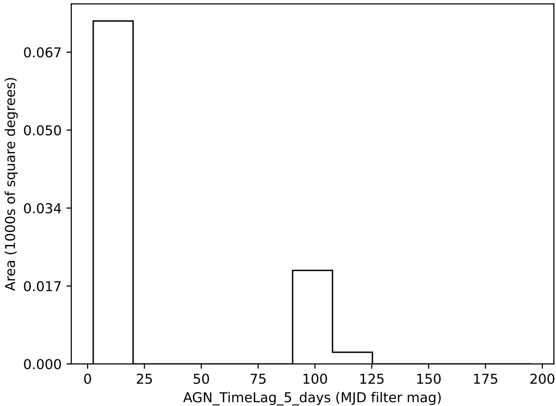
ddf_loaded_half_fl1_v3.4_10yrs all bands: AGN_TimeLag_5_days
