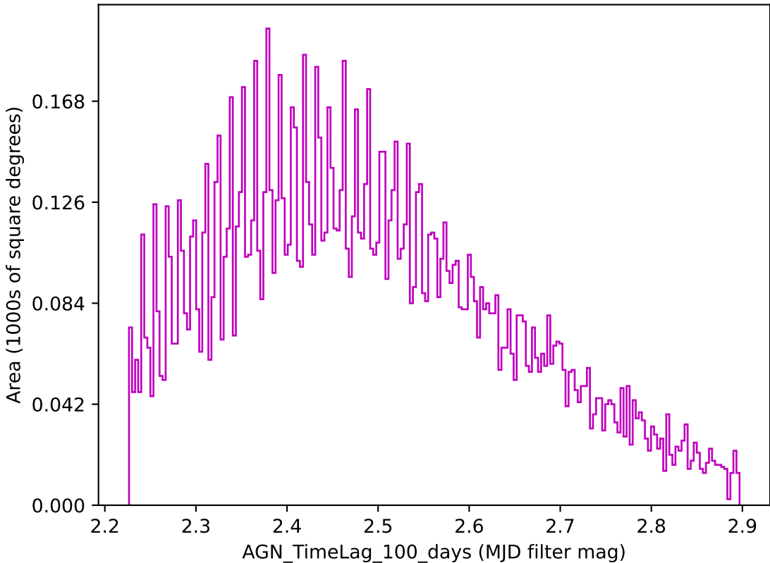
ddf_loaded_half_fl1_v3.4_10yrs z band: AGN_TimeLag_100_days
