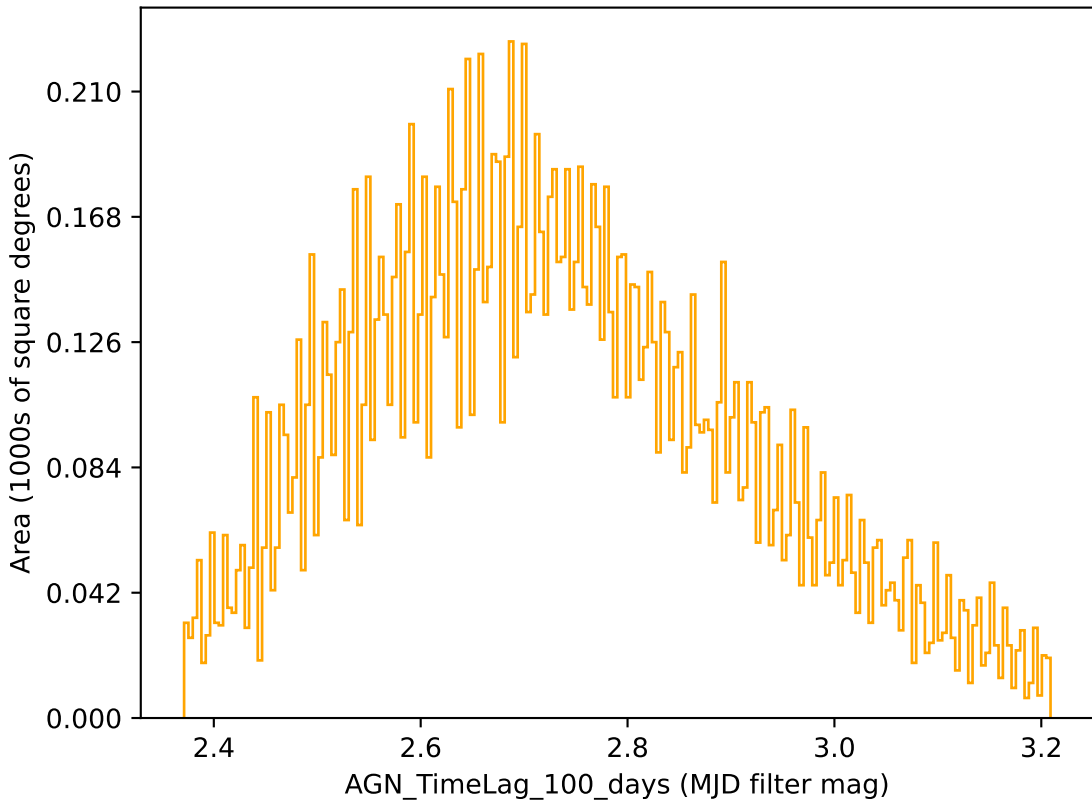
ddf_loaded_half_fl1_v3.4_10yrs r band: AGN_TimeLag_100_days
