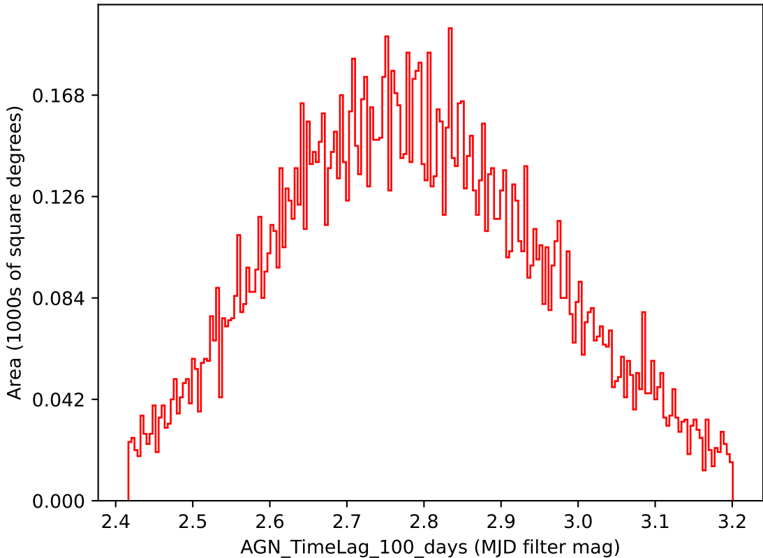
ddf_loaded_half_fl1_v3.4_10yrs i band: AGN_TimeLag_100_days
