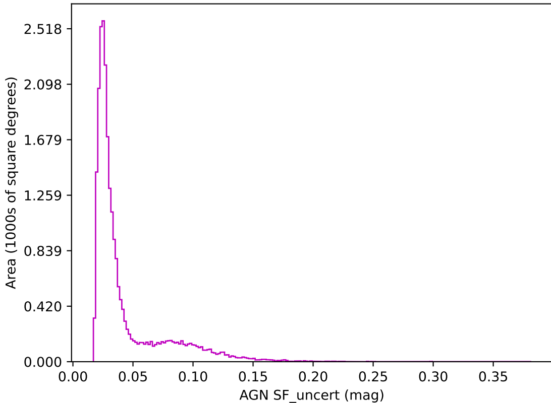
ddf_loaded_half_fl1_v3.4_10yrs z band: AGN SF_uncert
