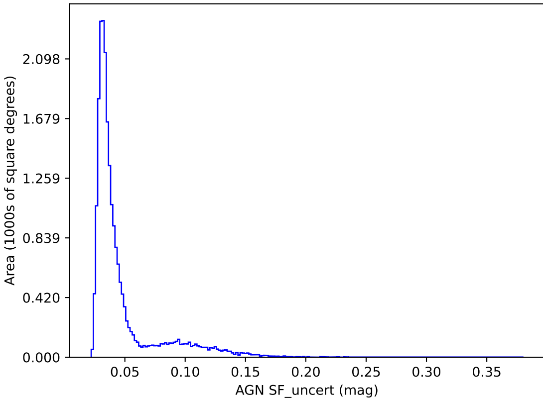
ddf_loaded_half_fl1_v3.4_10yrs y band: AGN SF_uncert
