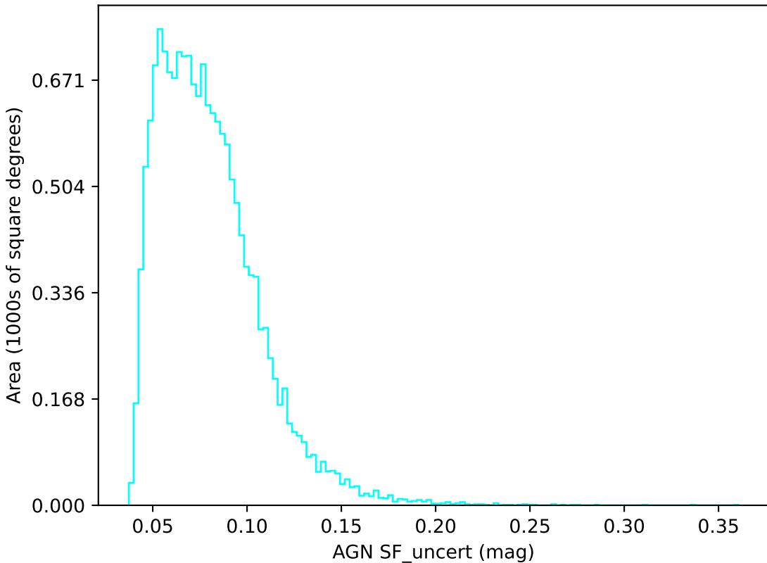
ddf_loaded_half_fl1_v3.4_10yrs u band: AGN SF_uncert
