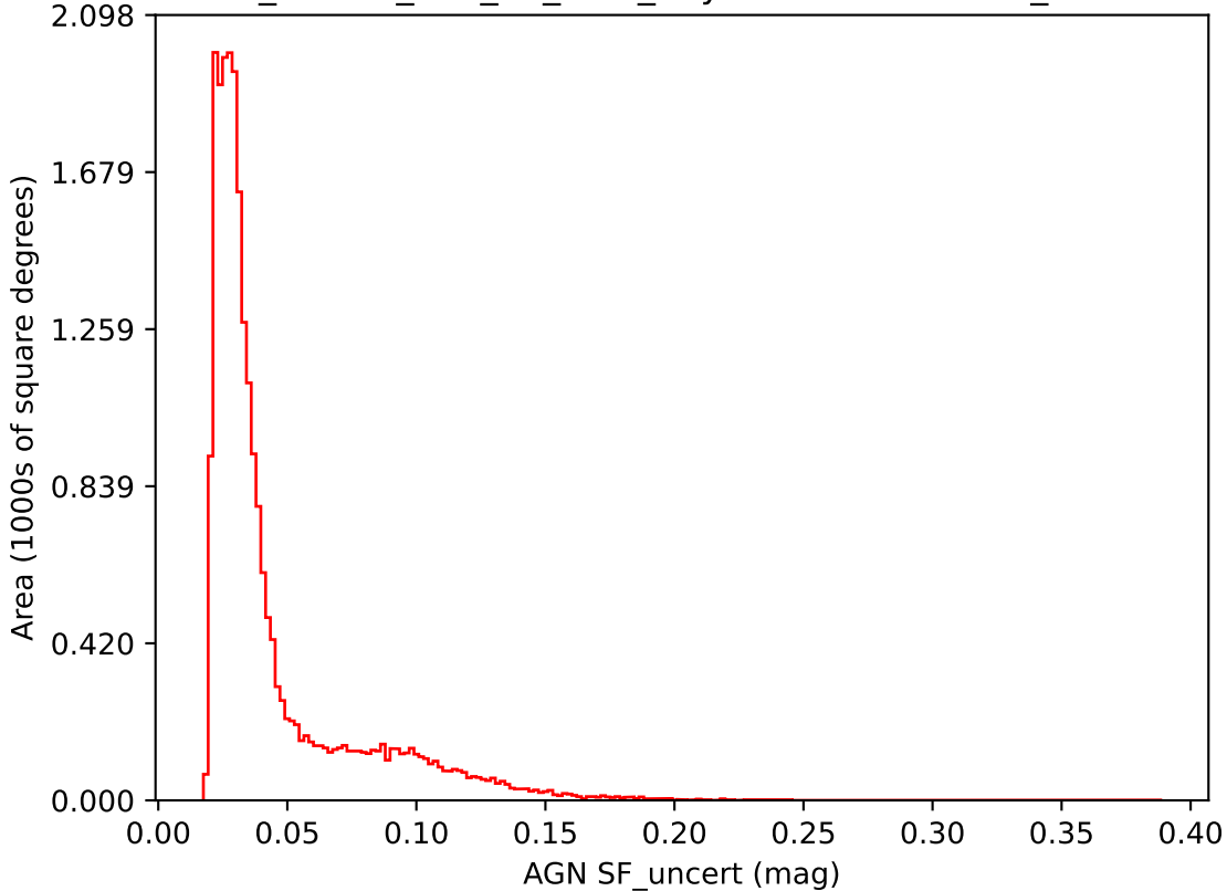
ddf_loaded_half_fl1_v3.4_10yrs i band: AGN SF_uncert
