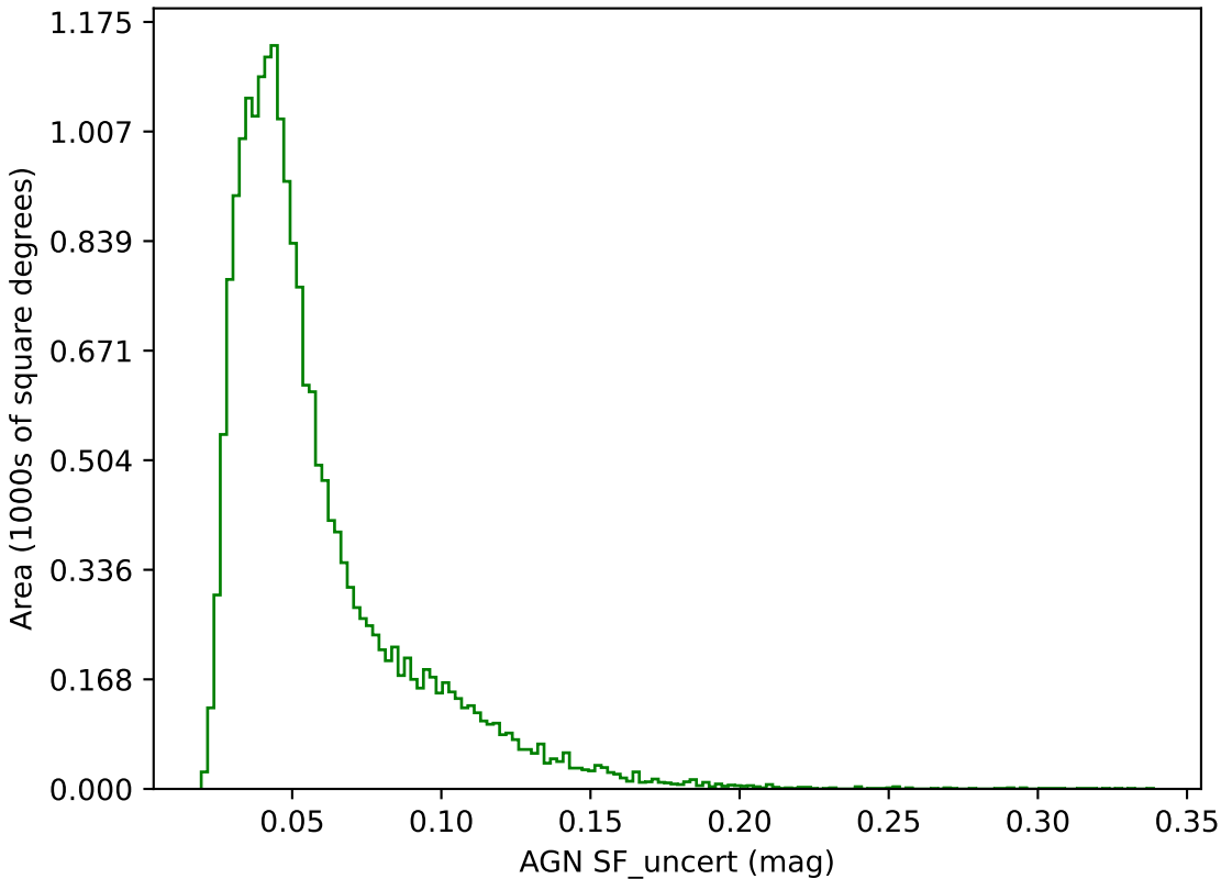
ddf_loaded_half_fl1_v3.4_10yrs g band: AGN SF_uncert
