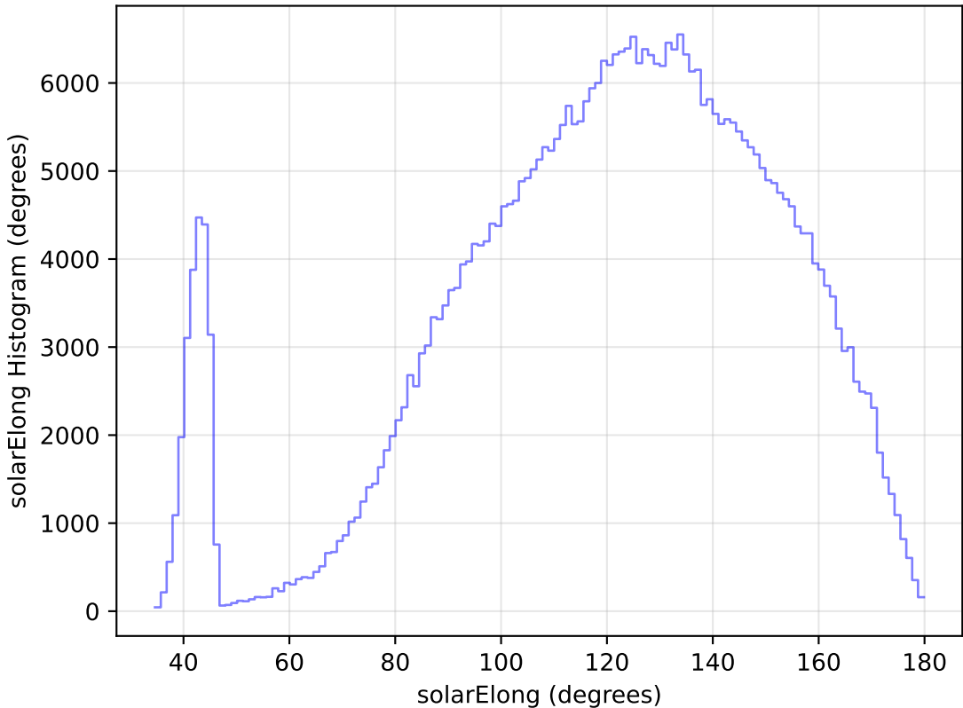
ddf_loaded_half_fl1_v3.4_10yrs WFD z band: solarElong Histogram
