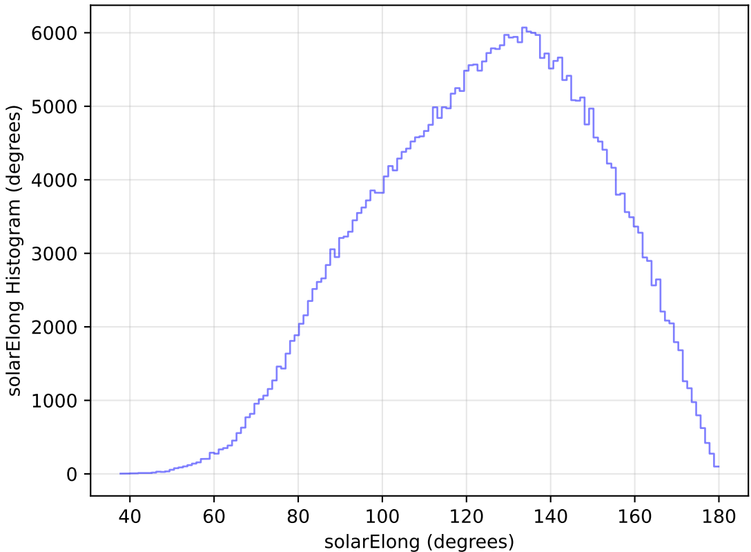
ddf_loaded_half_fl1_v3.4_10yrs WFD y band: solarElong Histogram
