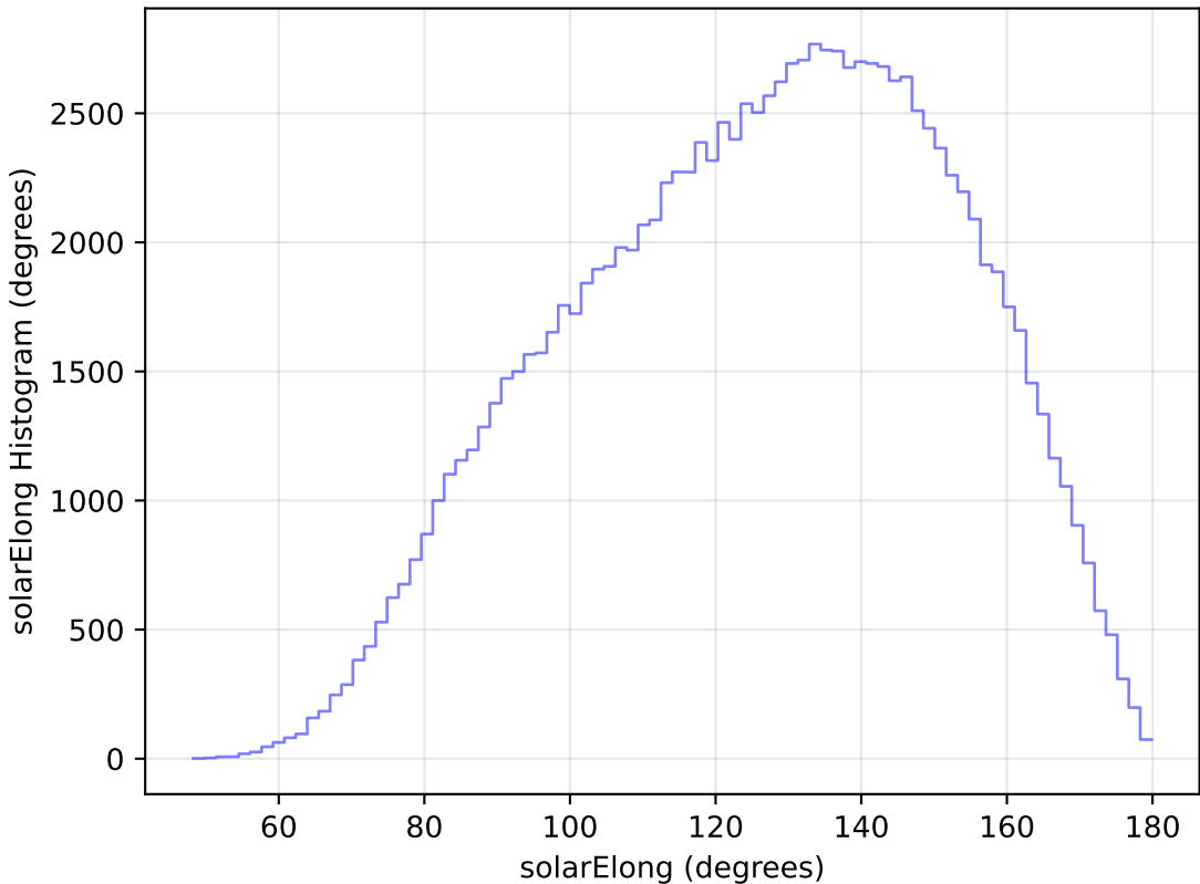
ddf_loaded_half_fl1_v3.4_10yrs WFD u band: solarElong Histogram
