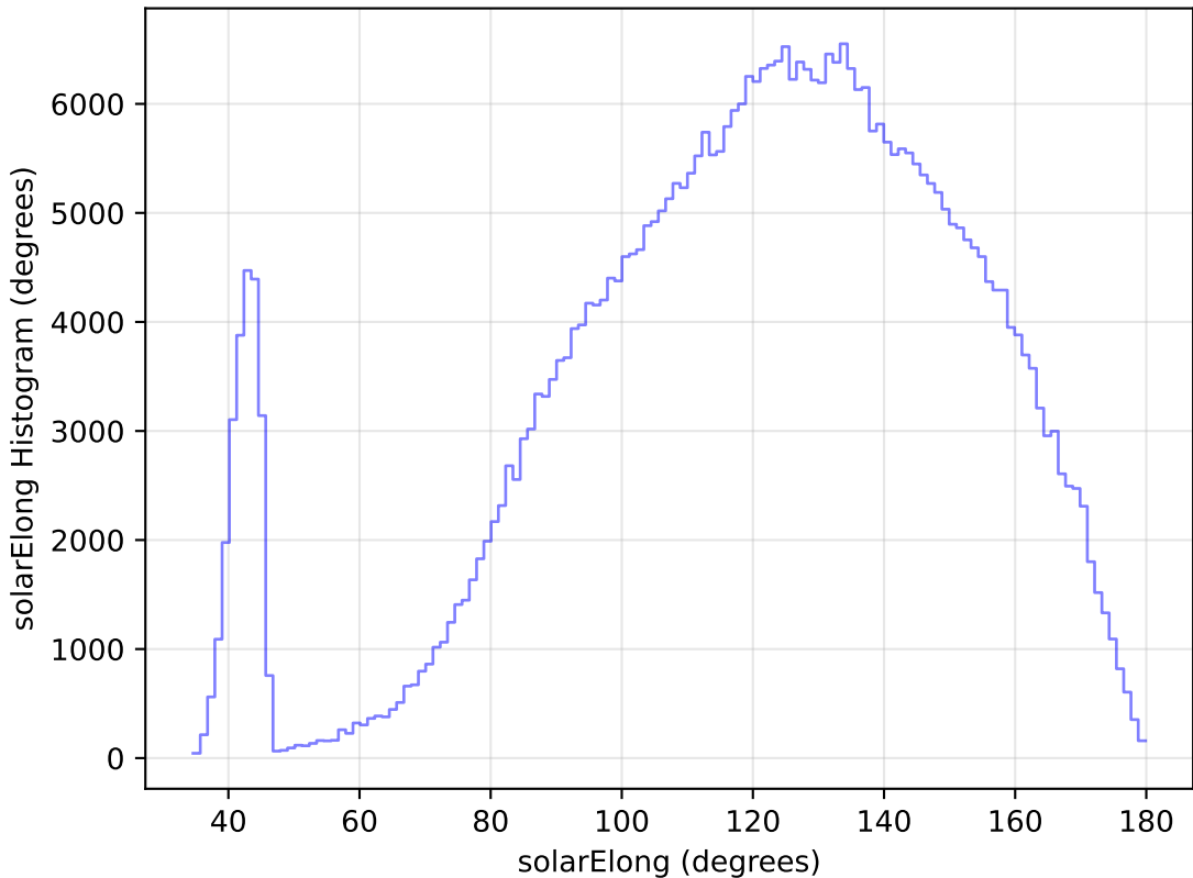
ddf_loaded_half_fl1_v3.4_10yrs All sky z band: solarElong Histogram
