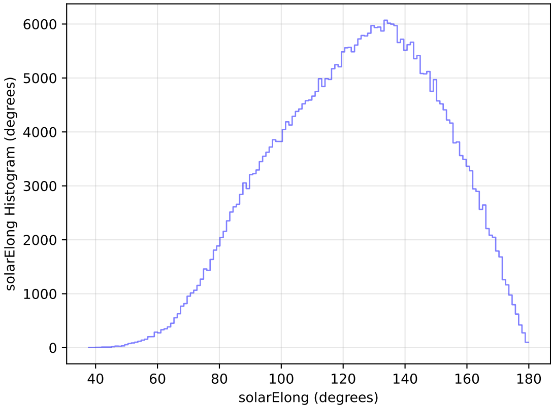
ddf_loaded_half_fl1_v3.4_10yrs All sky y band: solarElong Histogram
