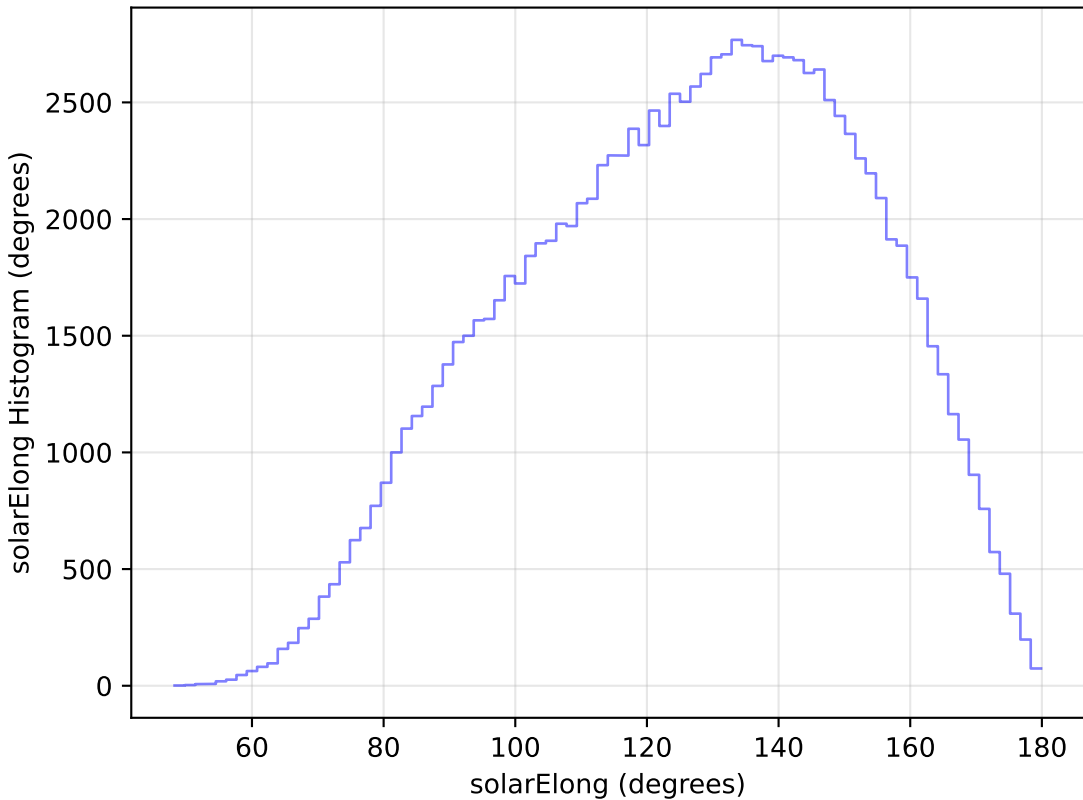
ddf_loaded_half_fl1_v3.4_10yrs All sky u band: solarElong Histogram
