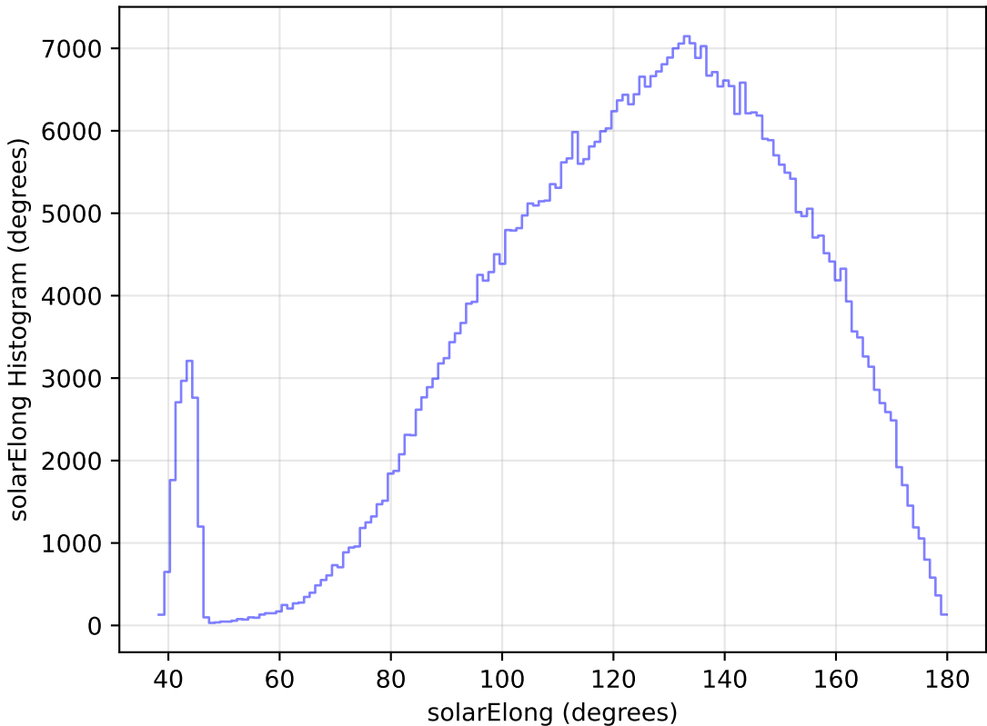
ddf_loaded_half_fl1_v3.4_10yrs All sky r band: solarElong Histogram
