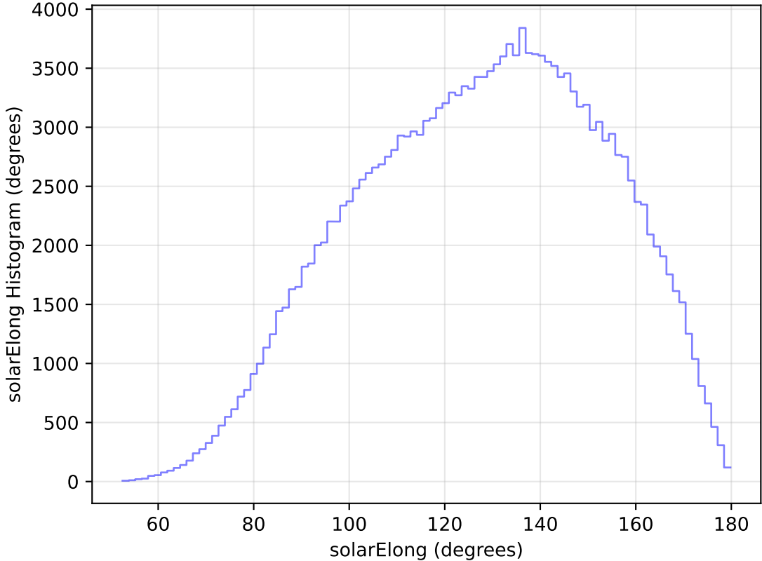
ddf_loaded_half_fl1_v3.4_10yrs All sky g band: solarElong Histogram
