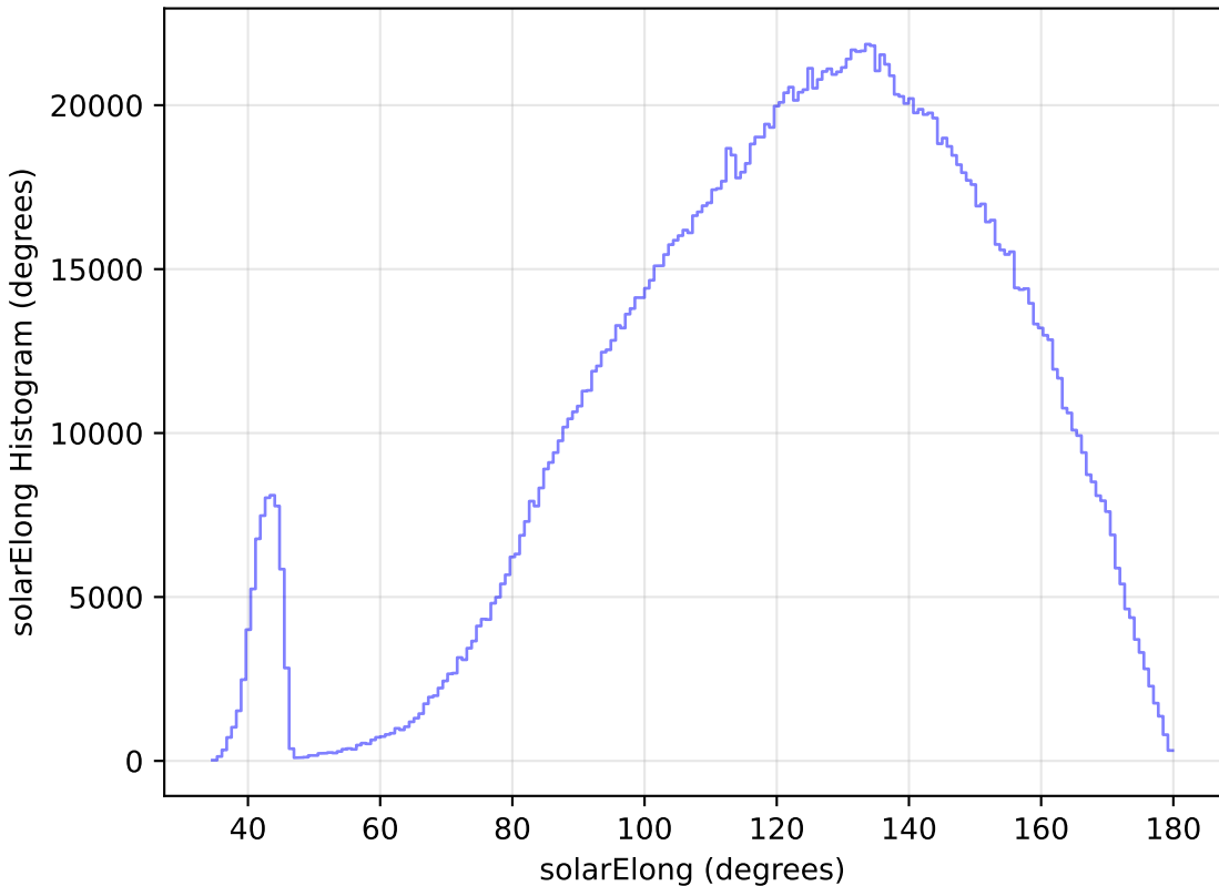
ddf_loaded_half_fl1_v3.4_10yrs All sky all bands: solarElong Histogram
