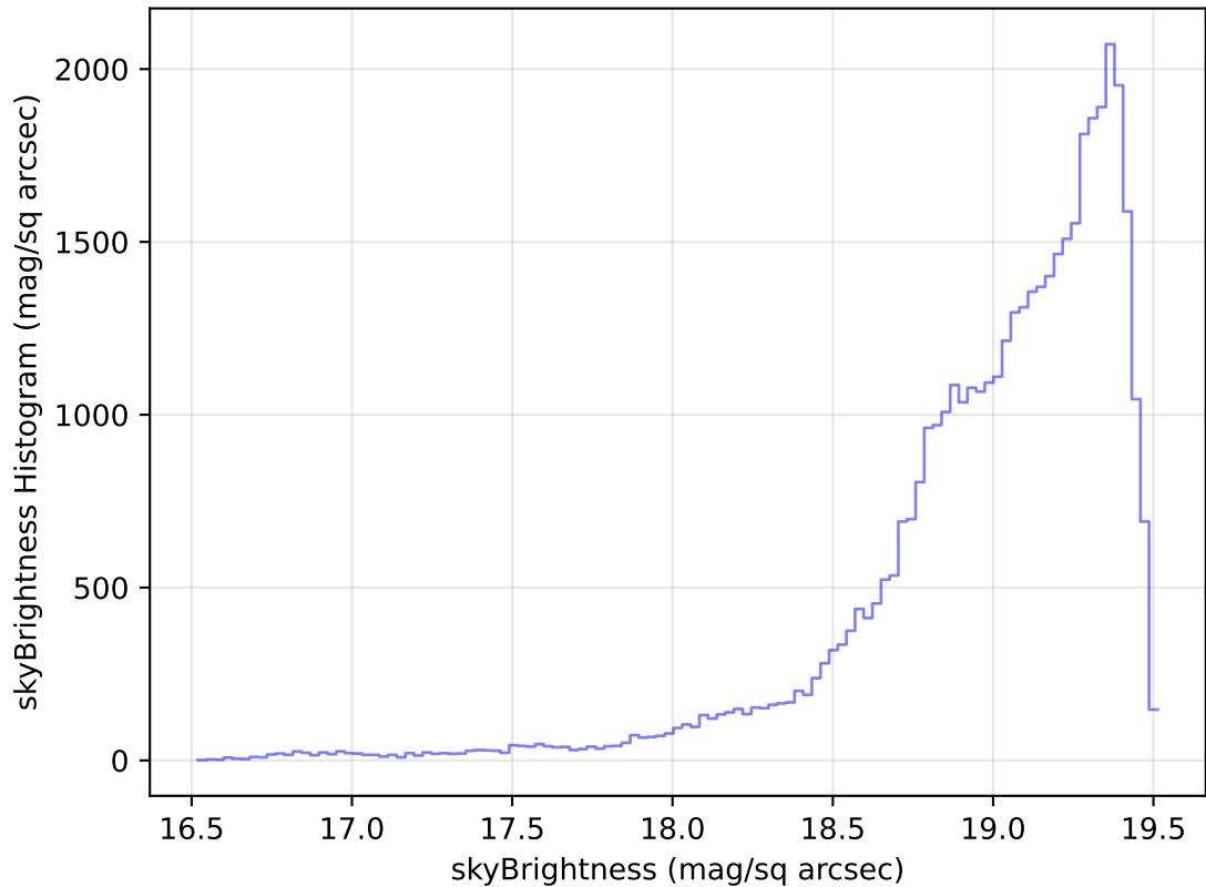
ddf_loaded_half_fl1_v3.4_10yrs Yr 1 z band: skyBrightness Histogram
