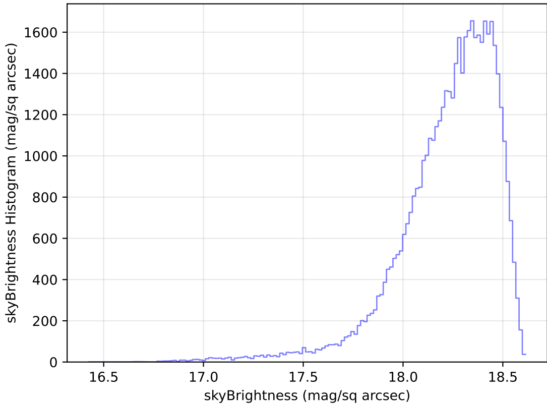
ddf_loaded_half_fl1_v3.4_10yrs Yr 1 y band: skyBrightness Histogram
