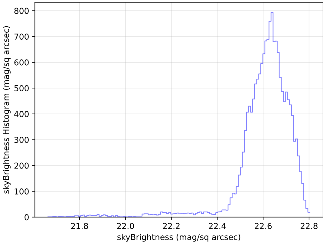
ddf_loaded_half_fl1_v3.4_10yrs Yr 1 u band: skyBrightness Histogram
