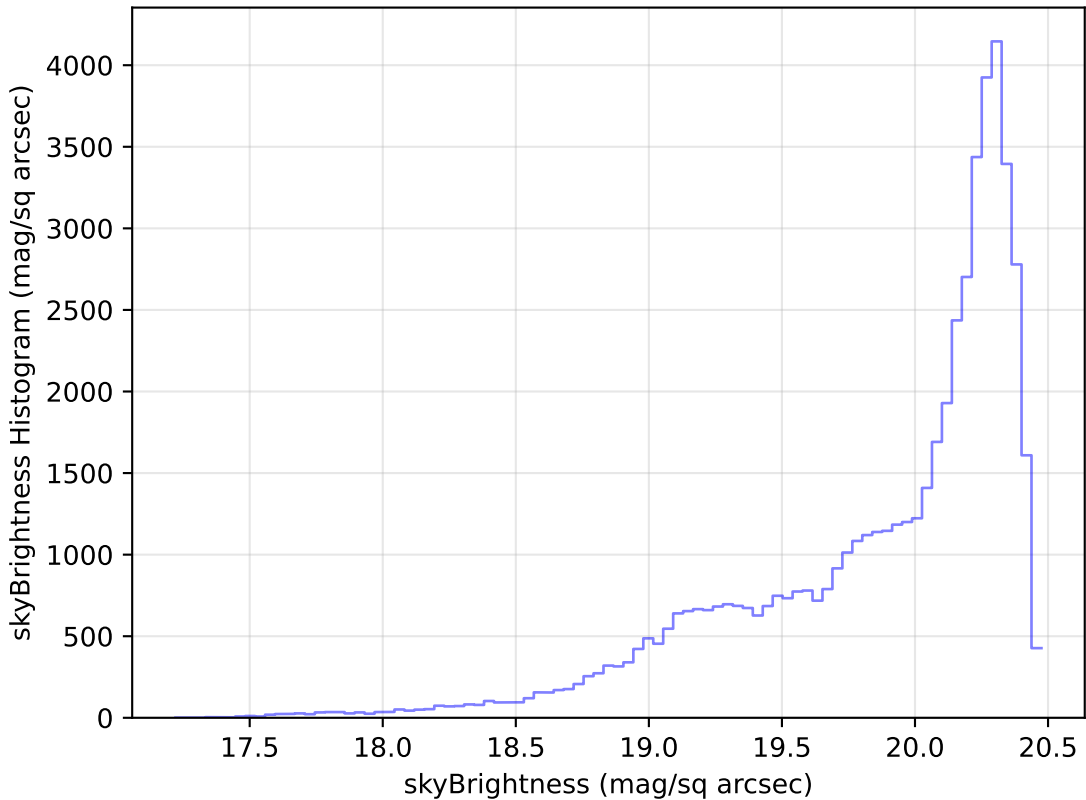
ddf_loaded_half_fl1_v3.4_10yrs Yr 1 i band: skyBrightness Histogram
