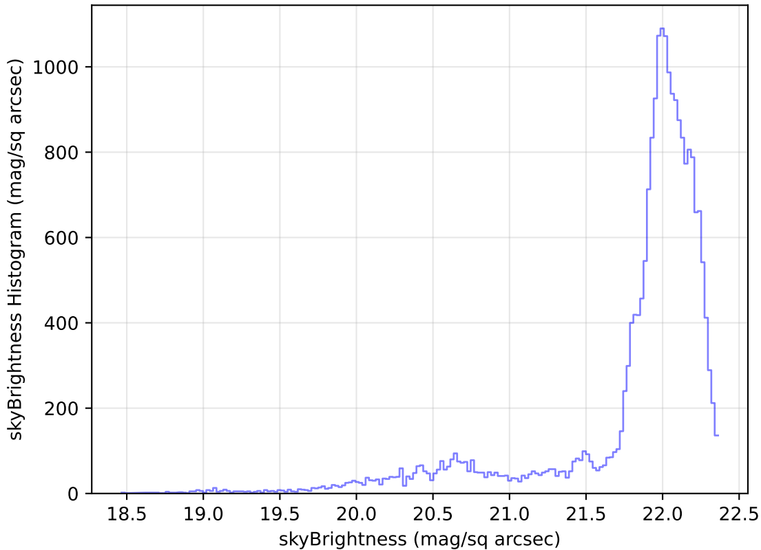
ddf_loaded_half_fl1_v3.4_10yrs Yr 1 g band: skyBrightness Histogram
