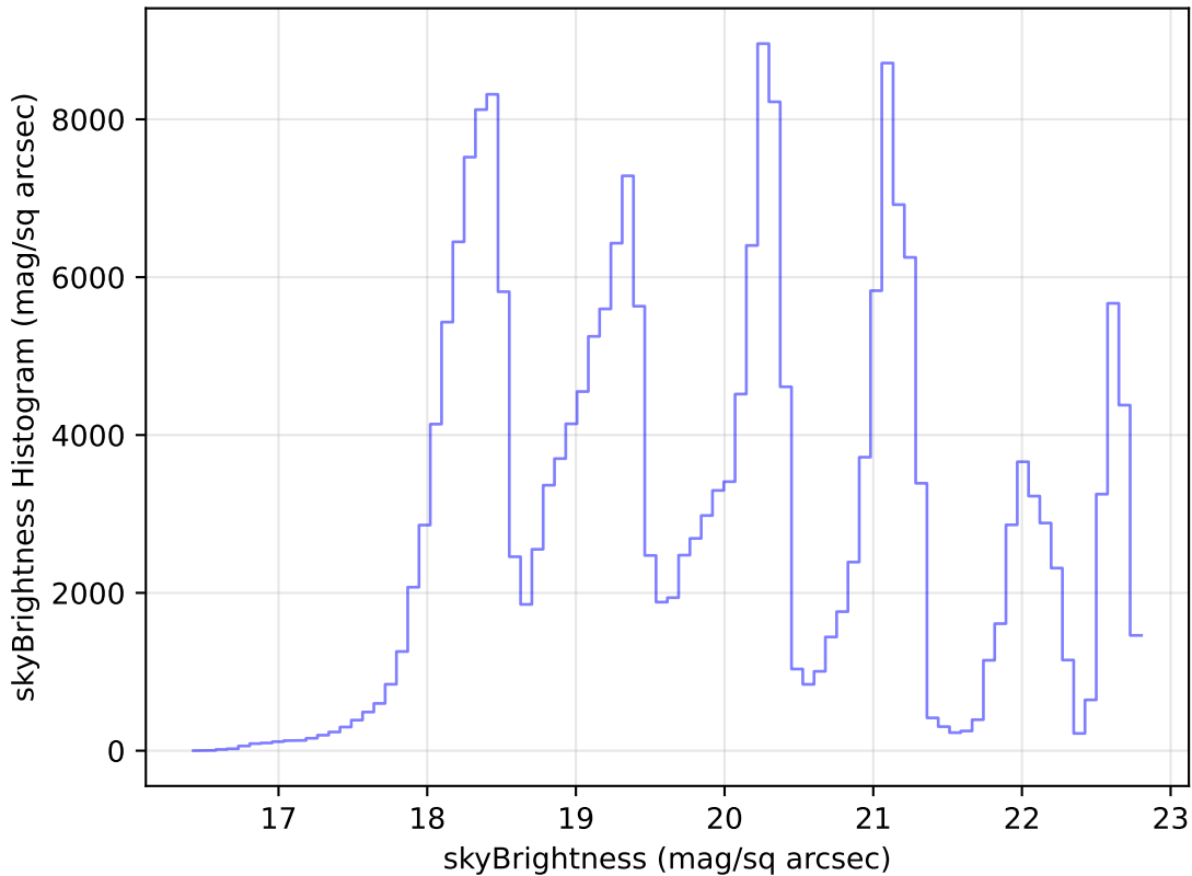
ddf_loaded_half_fl1_v3.4_10yrs Yr 1 all bands: skyBrightness Histogram
