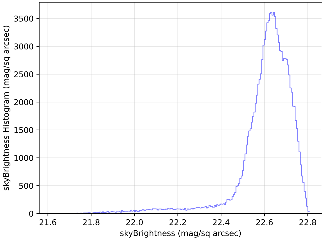
ddf_loaded_half_fl1_v3.4_10yrs WFD u band: skyBrightness Histogram
