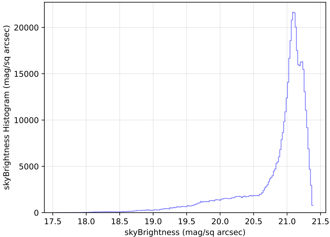
ddf_loaded_half_fl1_v3.4_10yrs WFD r band: skyBrightness Histogram
