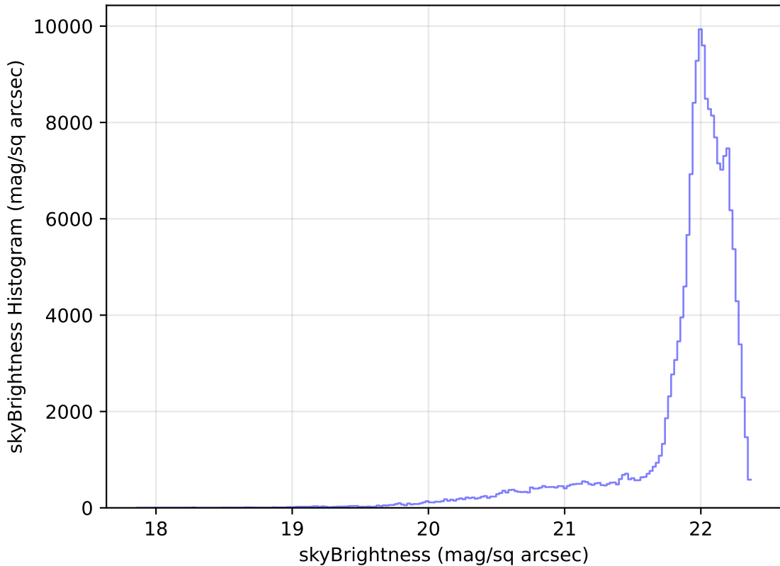
ddf_loaded_half_fl1_v3.4_10yrs WFD g band: skyBrightness Histogram
