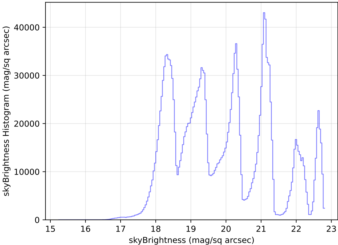
ddf_loaded_half_fl1_v3.4_10yrs WFD all bands: skyBrightness Histogram
