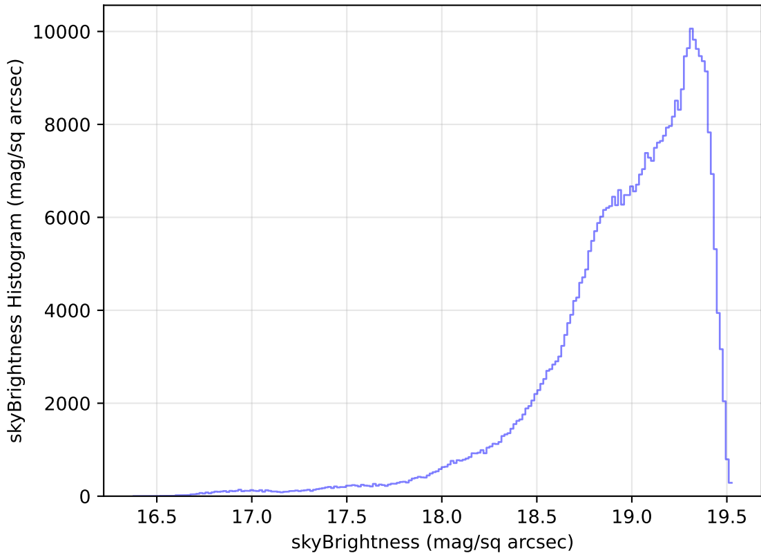
ddf_loaded_half_fl1_v3.4_10yrs All sky z band: skyBrightness Histogram
