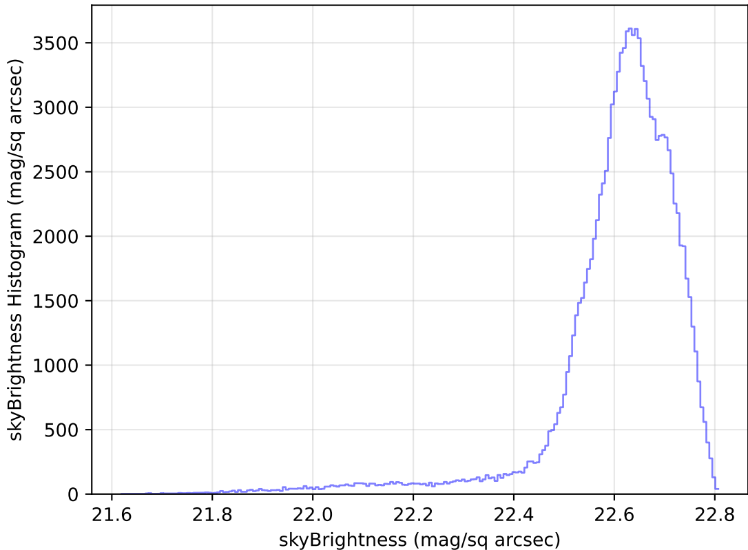
ddf_loaded_half_fl1_v3.4_10yrs All sky u band: skyBrightness Histogram
