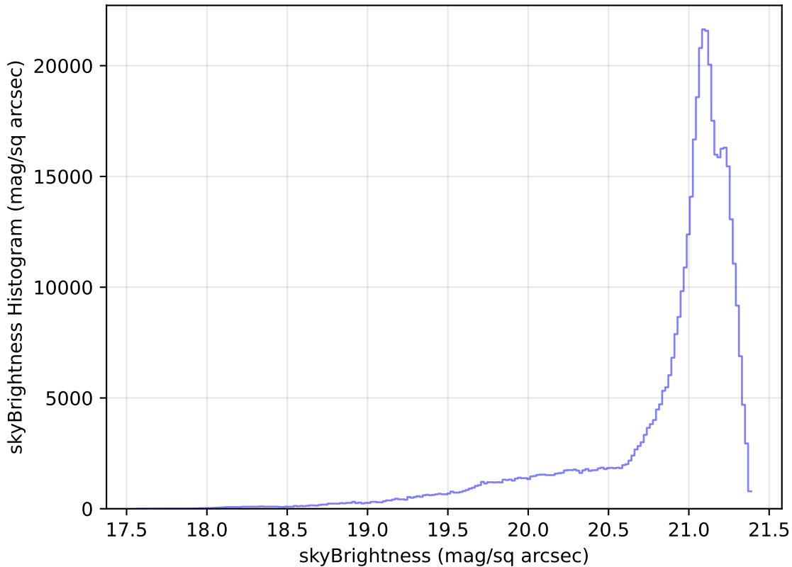
ddf_loaded_half_fl1_v3.4_10yrs All sky r band: skyBrightness Histogram
