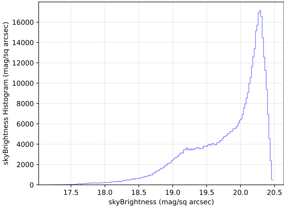
ddf_loaded_half_fl1_v3.4_10yrs All sky i band: skyBrightness Histogram
