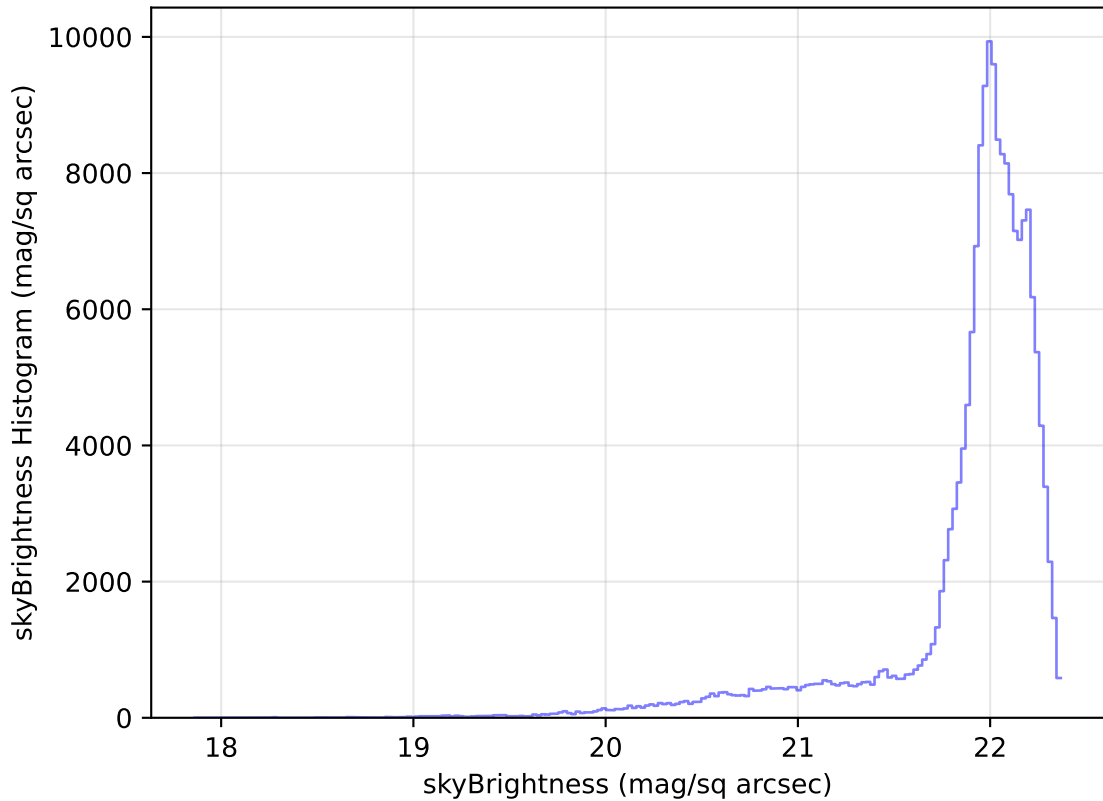
ddf_loaded_half_fl1_v3.4_10yrs All sky g band: skyBrightness Histogram
