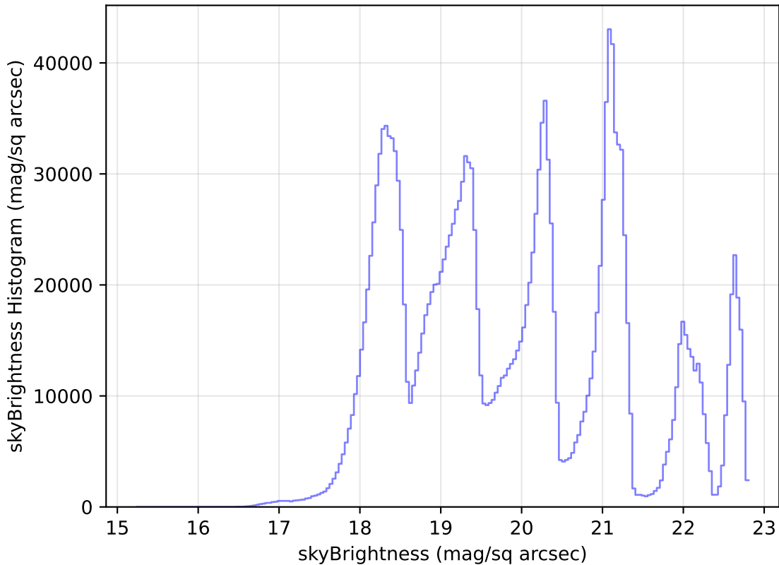
ddf_loaded_half_fl1_v3.4_10yrs All sky all bands: skyBrightness Histogram
