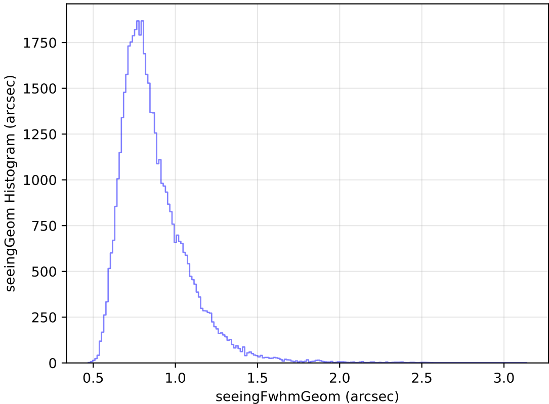
ddf_loaded_half_fl1_v3.4_10yrs Yr 1 y band: seeingGeom Histogram
