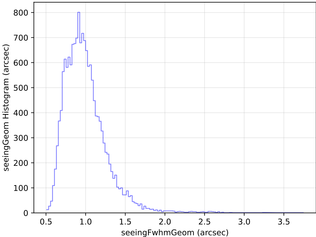
ddf_loaded_half_fl1_v3.4_10yrs Yr 1 u band: seeingGeom Histogram
