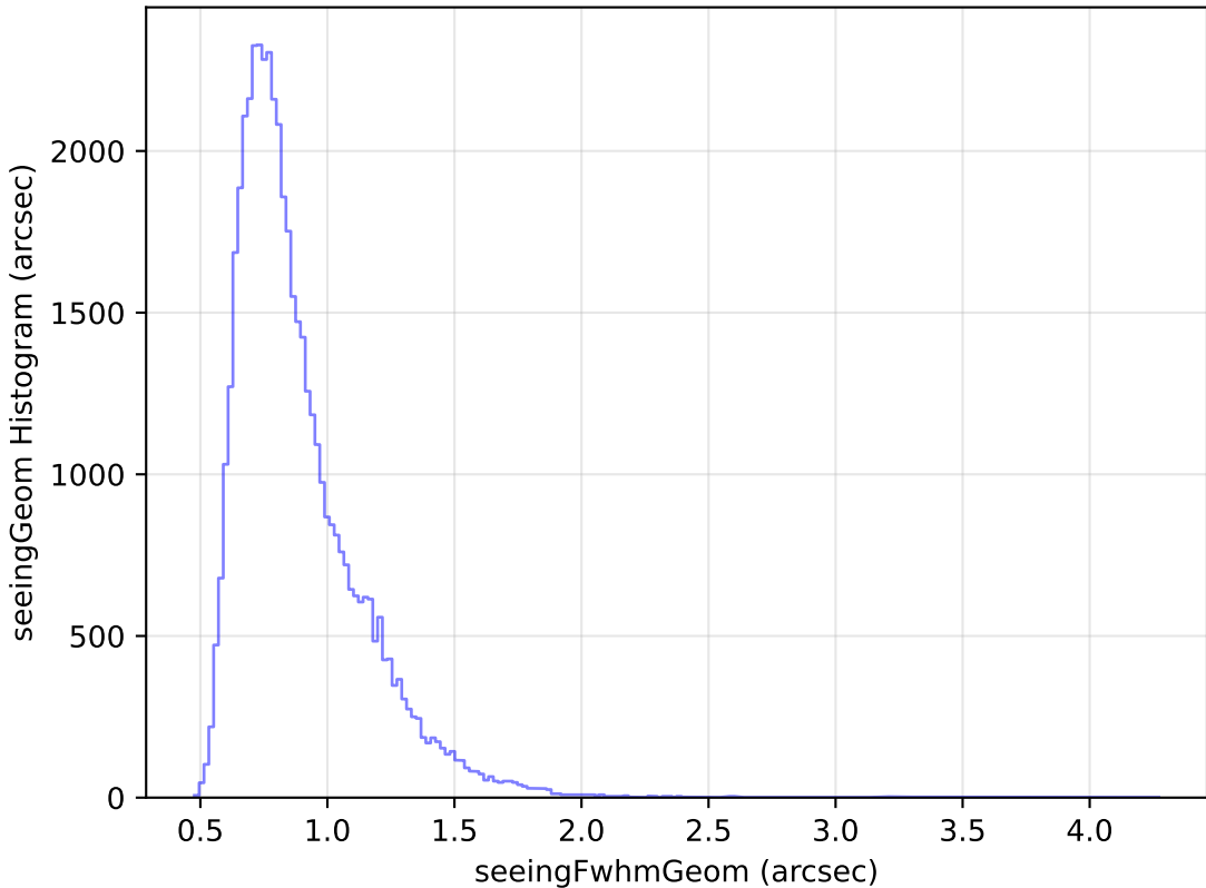
ddf_loaded_half_fl1_v3.4_10yrs Yr 1 r band: seeingGeom Histogram
