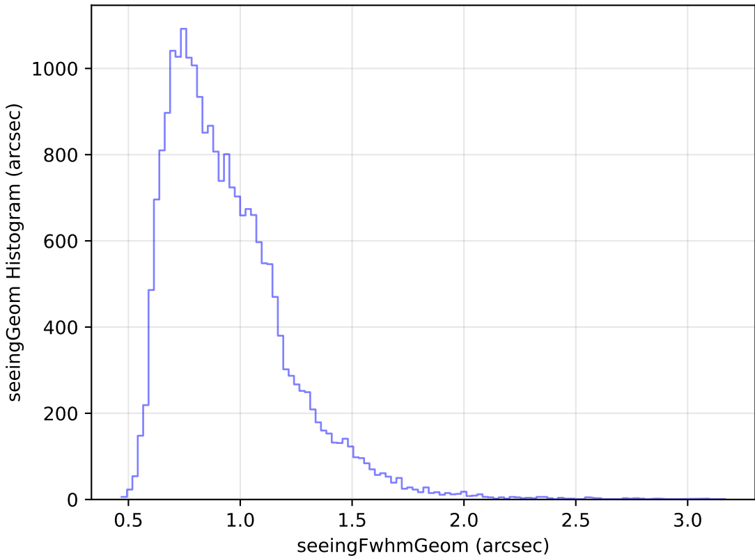
ddf_loaded_half_fl1_v3.4_10yrs Yr 1 g band: seeingGeom Histogram
