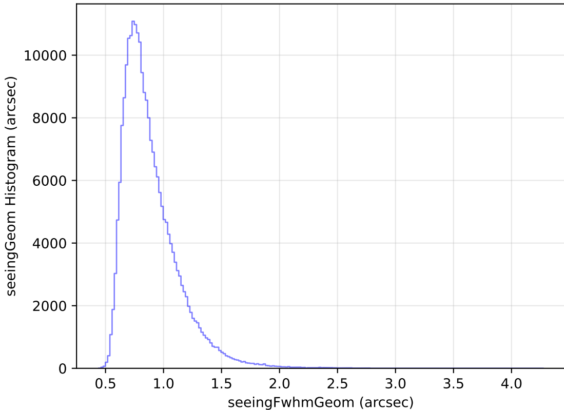
ddf_loaded_half_fl1_v3.4_10yrs Yr 1 all bands: seeingGeom Histogram
