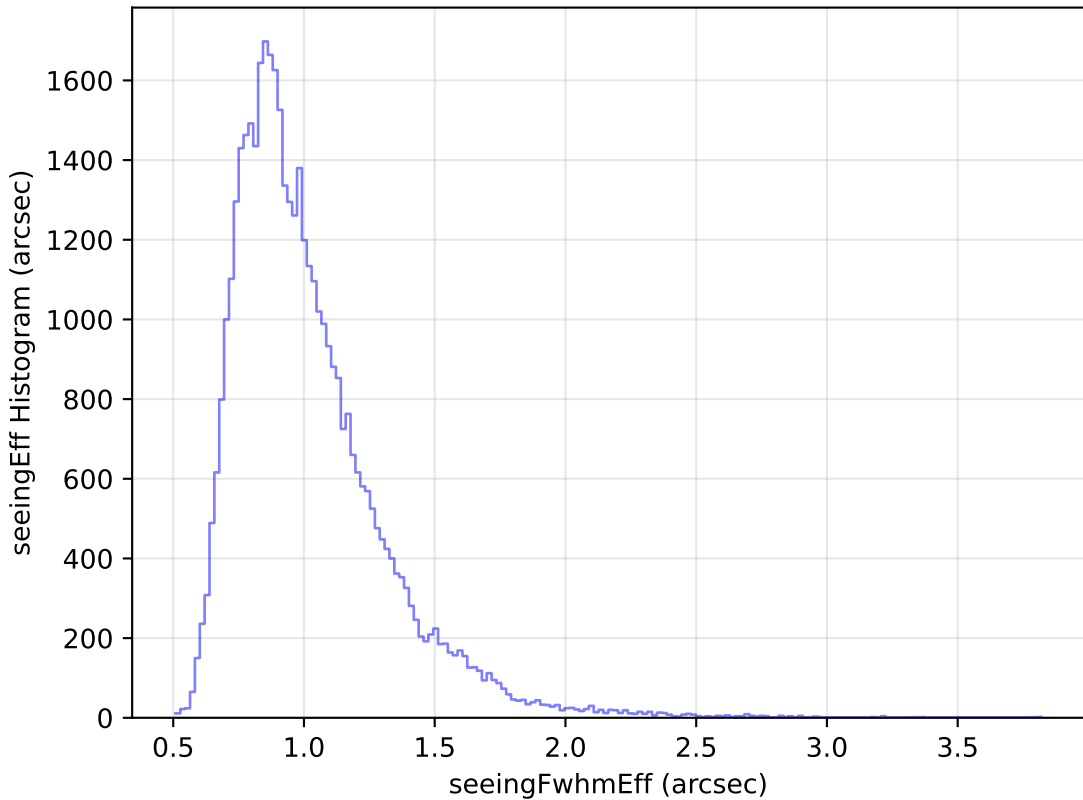
ddf_loaded_half_fl1_v3.4_10yrs Yr 1 z band: seeingEff Histogram
