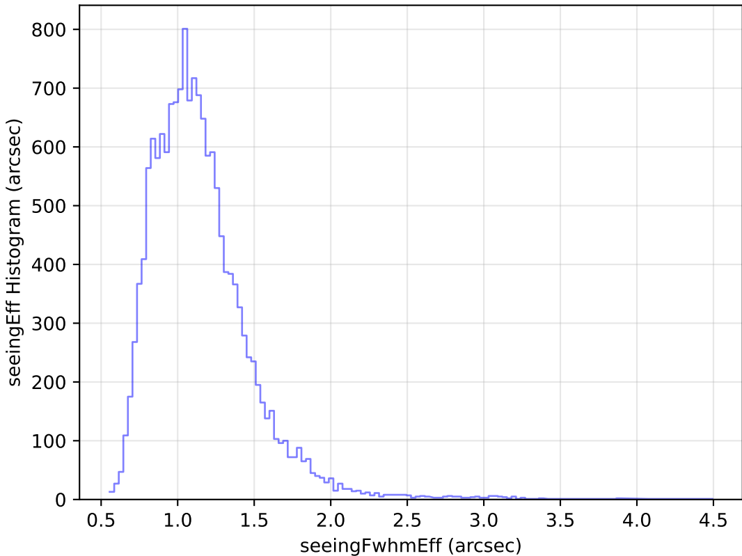
ddf_loaded_half_fl1_v3.4_10yrs Yr 1 u band: seeingEff Histogram
