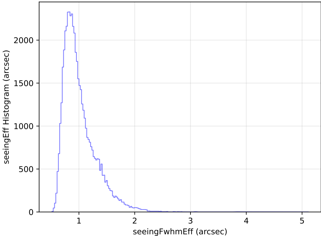
ddf_loaded_half_fl1_v3.4_10yrs Yr 1 r band: seeingEff Histogram
