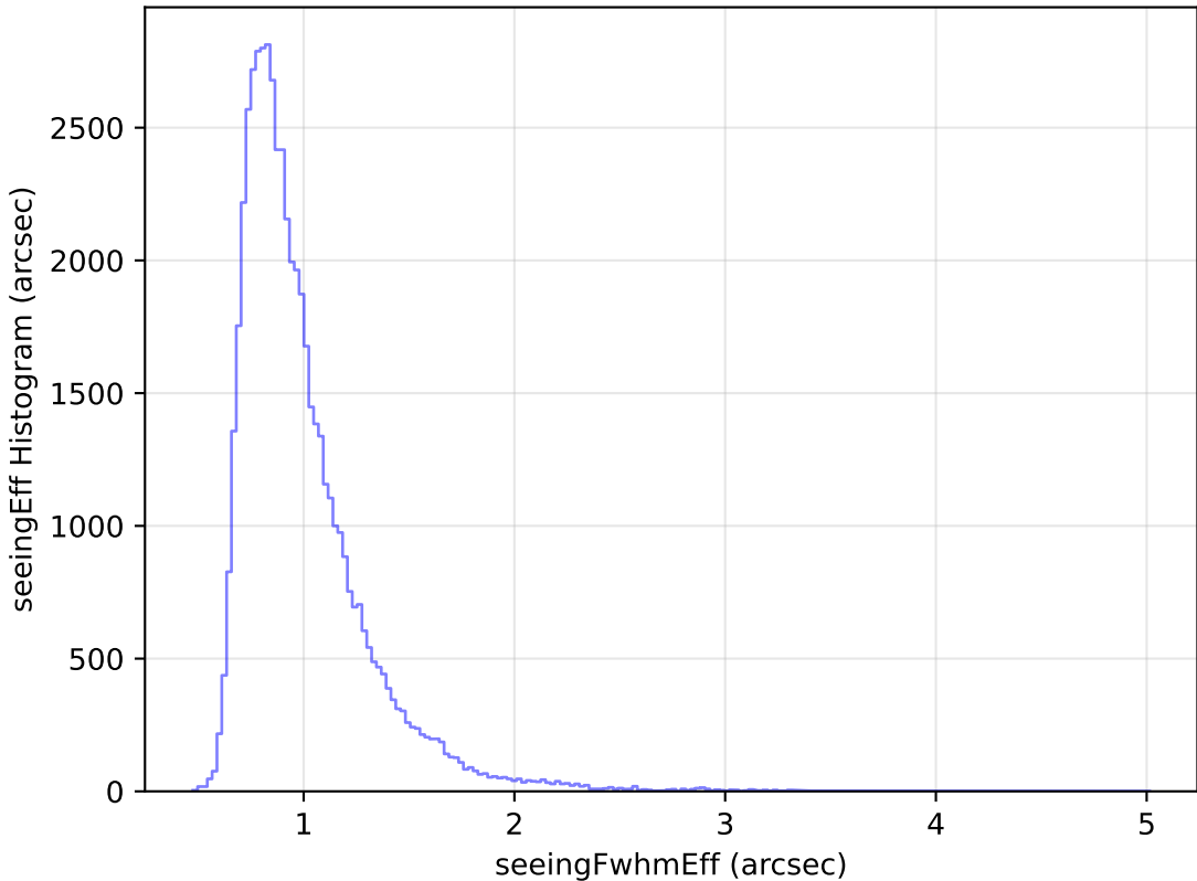
ddf_loaded_half_fl1_v3.4_10yrs Yr 1 i band: seeingEff Histogram
