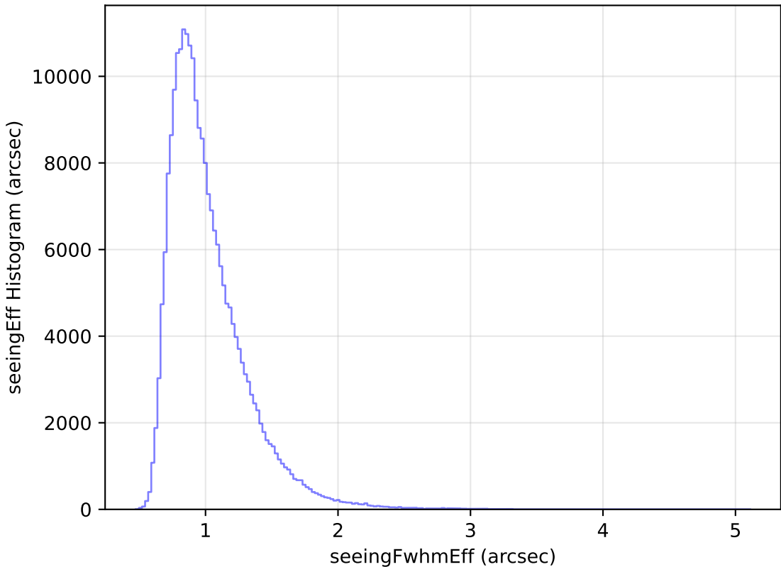
ddf_loaded_half_fl1_v3.4_10yrs Yr 1 all bands: seeingEff Histogram
