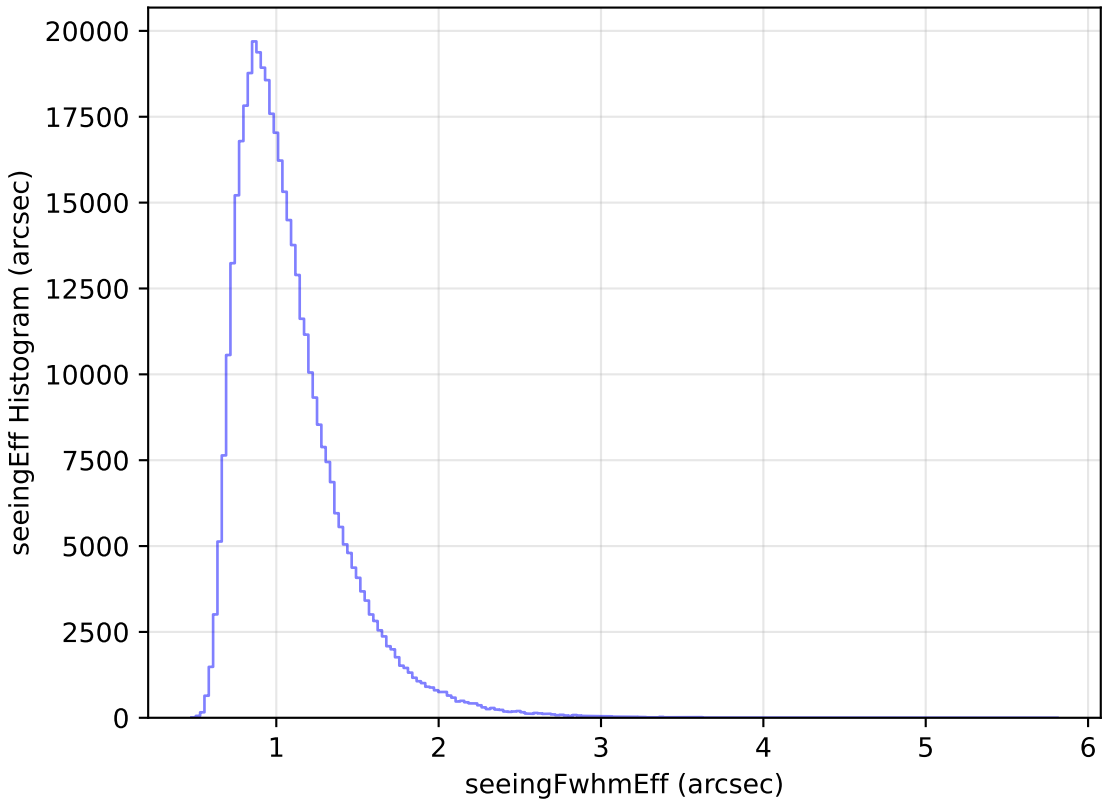
ddf_loaded_half_fl1_v3.4_10yrs WFD z band: seeingEff Histogram
