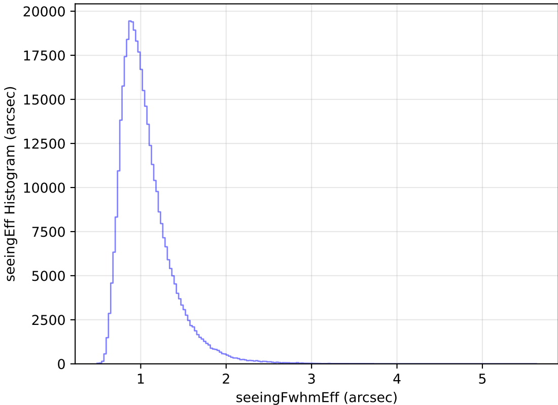
ddf_loaded_half_fl1_v3.4_10yrs WFD y band: seeingEff Histogram
