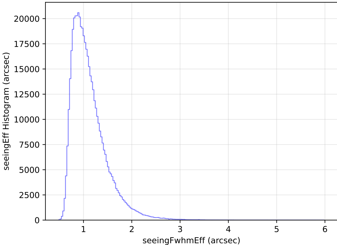
ddf_loaded_half_fl1_v3.4_10yrs WFD r band: seeingEff Histogram
